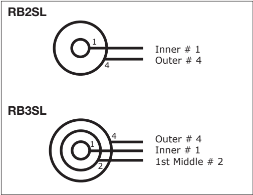
Gas valve and burner ring matching.
